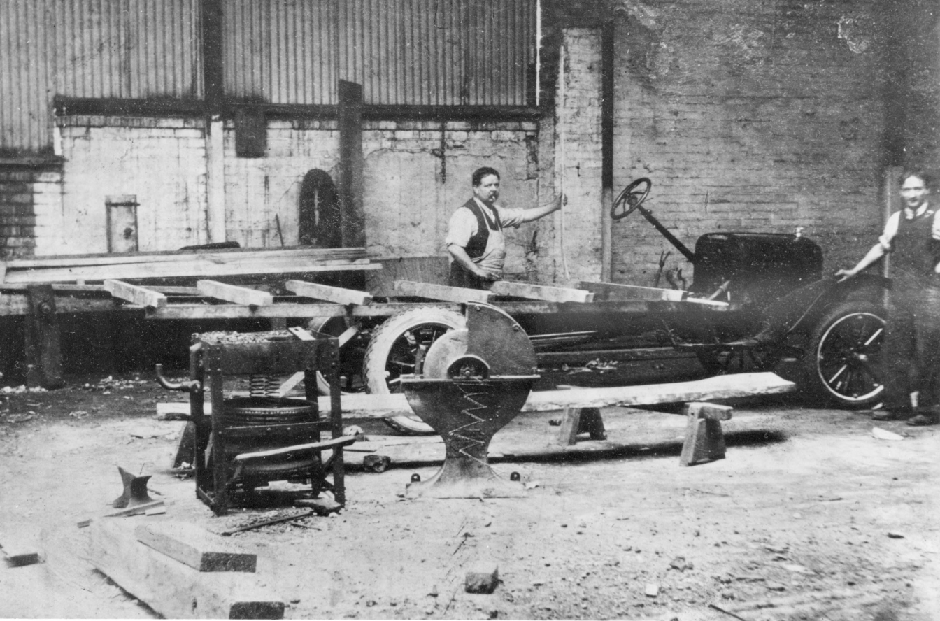
1921 Chassis for motor caravan at Gosta Green Factory
